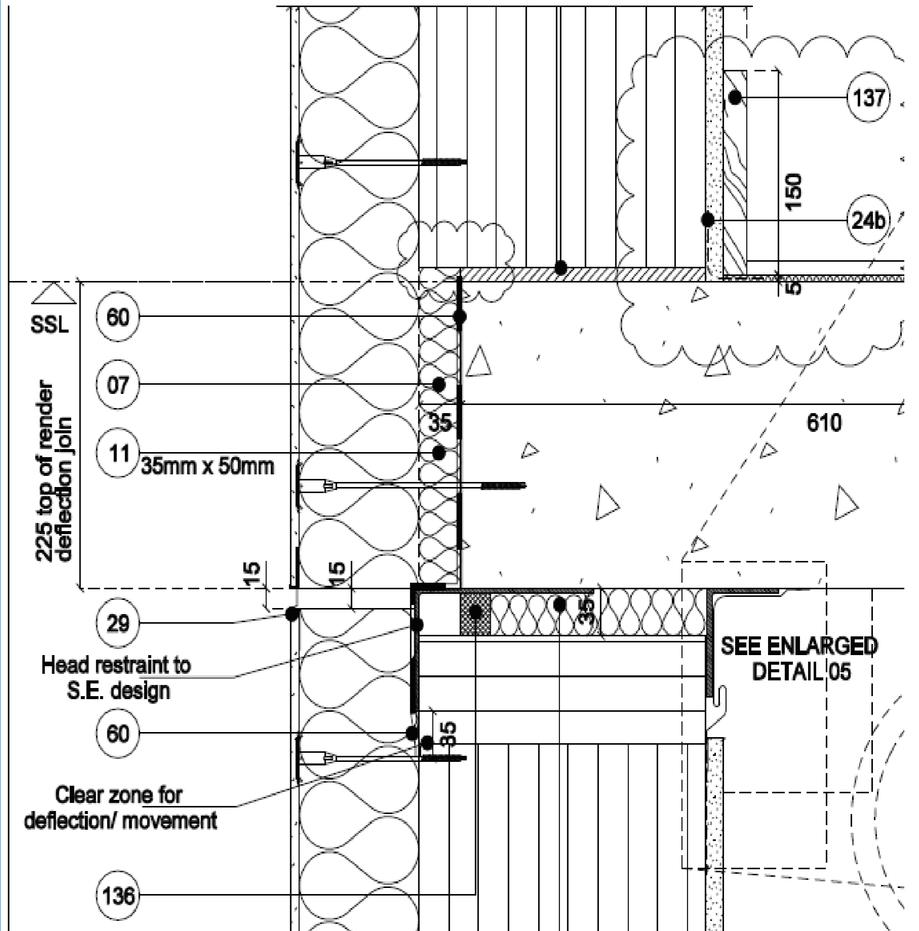
Section through slab showing Thermoplan blocks projecting
