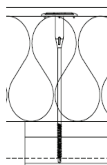
Figures: Fixing the wood-fibre board and the thermally broken fasteners
