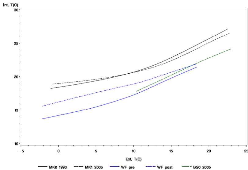
Daily Average Bedroom Temp, vs Ext. Temp.
